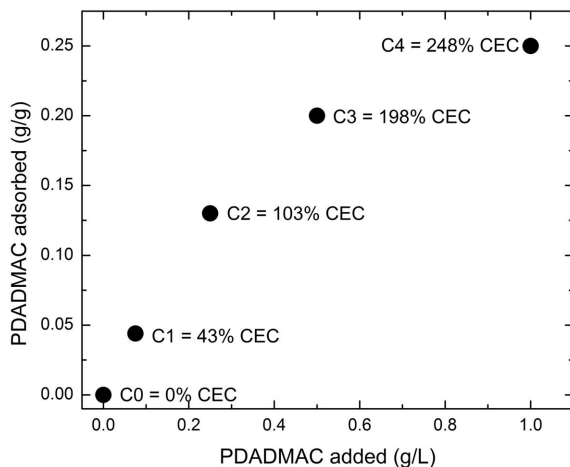
Figure 2. Adsorption of poly-DADMAC (0–1 g/L added) on unaltered (oxidized) SWa-1 (1.67 g/L) smectite samples C0 to C4, expressed as both the gravimetric amount adsorbed (std. dev. = \pm 0.03\text{ g/g} ) and the fraction of CEC adsorbed.
